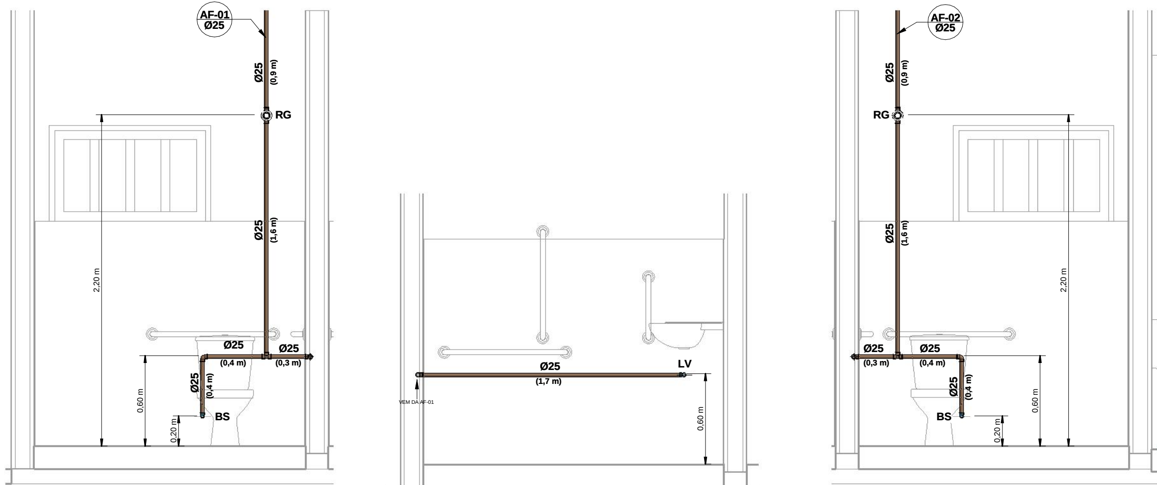
1 CORTE AF-01(BS) 1 : 25
