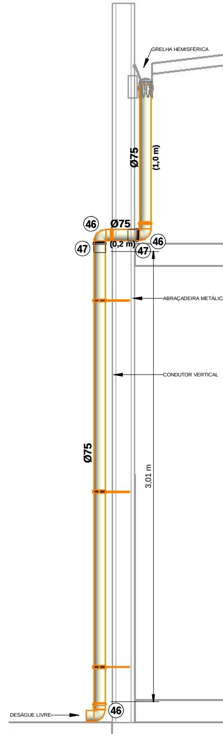
2 DET. CONDUCTOR VERTICAL 1 : 25
